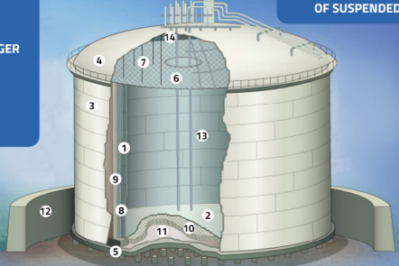
TANK ON GRADE OR ELEVATED
